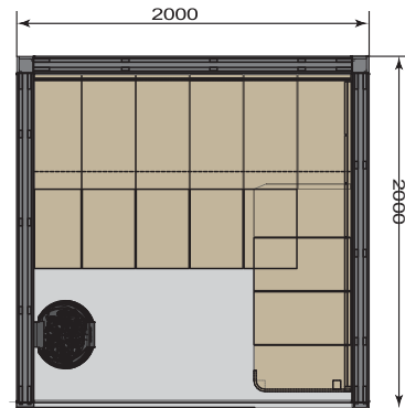
HSSHV2020
