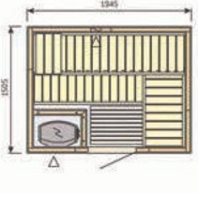
HVS2020
