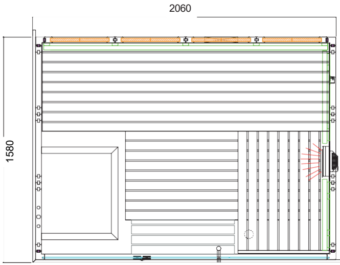
Harvia Himalaya Hybrid Küçük Kabin
