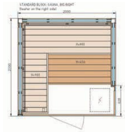
HSSHB2020ALD
