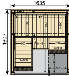
Variant View Köşe Tip Sauna HVS1616CVX
