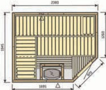
HVS2520R
